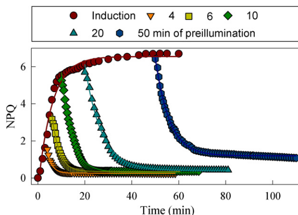
Fig. 6. Time course of nonphotochemical quenching (NPQ) induction and relaxation in Macrocytis pyrifera blades collected from the surface. Samples were exposed to approximately 60 min to 1000 \mu\text{mol photon m}^{-2} \text{ s}^{-1} and samples (in triplicate) were collected at 4, 6, 10, 20 and 50 min. These subsamples were maintained in darkness to evaluate NPQ relaxation. The data represent the average of the three replicates.
