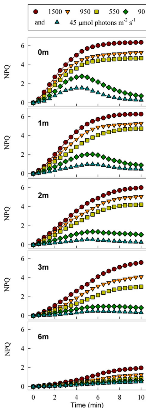
Fig. 2. Time course of nonphotochemical quenching (NPQ) in Macrocytis pyrifera blades collected from different depths. Triplicate samples of each depth were exposed to five different irradiances. The data represent the average of the three replicates.
