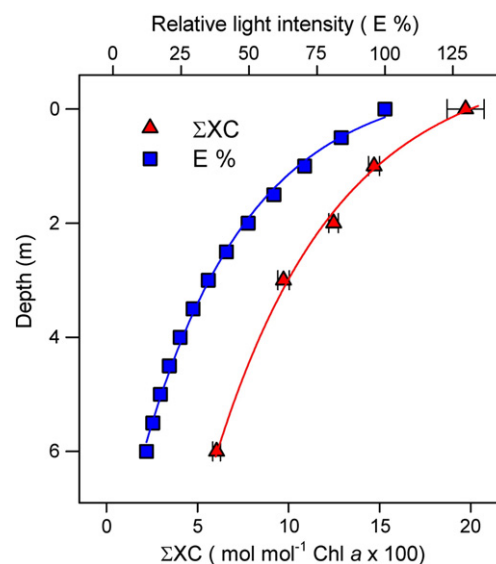
Fig. 1. Depth variation of the xanthophyll cycle pigment pool ( \Sigma XC ) in Macrocystis pyrifera blades and irradiance (E) in the water column. Irradiance is normalized to the intensity reaching the surface. Light data was fitted to the Lambert–Beer model of reduction of irradiance in the water column with an extinction coefficient ( k_d ) of 0.4 \text{m}^{-1} (continuous blue line). Also, \Sigma XC variation was modeled with an exponential model of reduction of this pool with depth (continuous red line).
