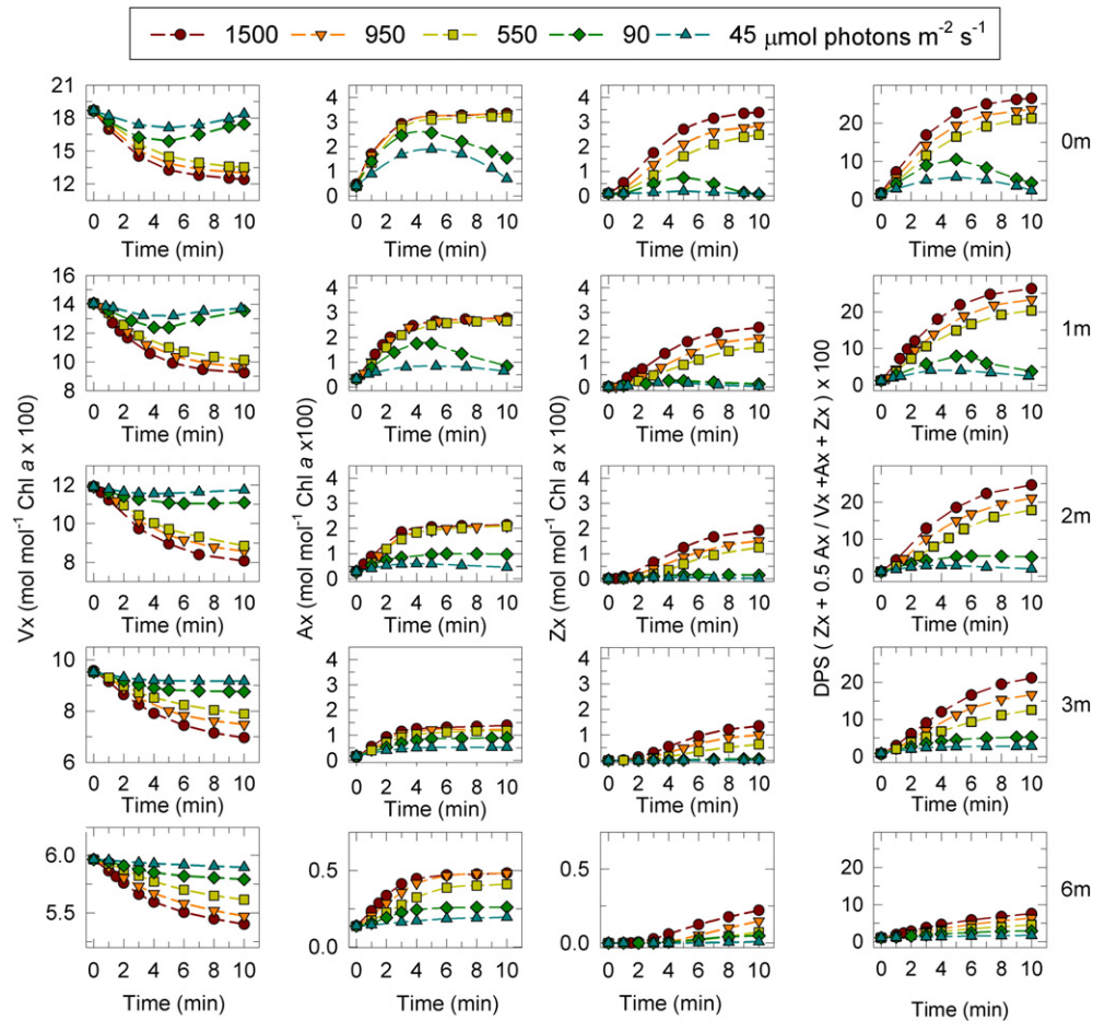
Fig. 3. Time course of the change of violaxanthin (Vx), antheraxanthin (Ax) and zeaxanthin (Zx) concentration in Macrocytis pyrifera blades collected from different depths. The change of the de-epoxidation state of the XC pigment pool (DPS) is also presented. Triplicate samples of each depth were exposed to five different irradiances. The data represent the average of the three replicates. Note the change in the scale of the Y axis in graphs of each collection depth.
